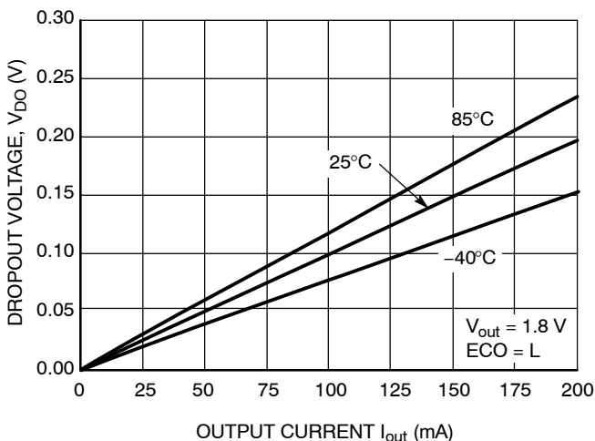
Figure 22. Dropout Voltage vs. Output Current
